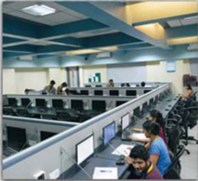
Image Processing
