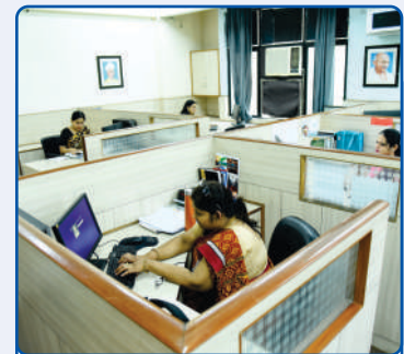
Faculty Nodes
